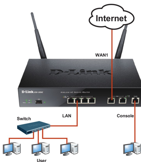
Figure 5. Basic Cabling Example
