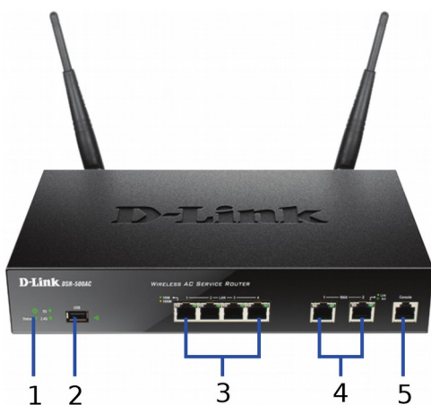
Figure 1. DSR-500AC Front Panel
