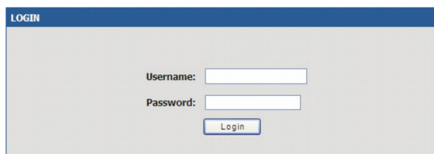
Figure 7. Authentication Message
