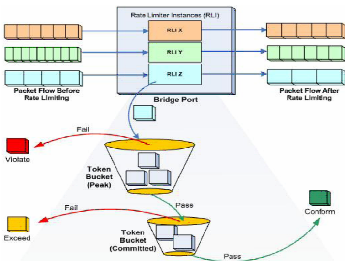
Рисунок 10-3. Two Rate Three Color Marking (TRTCM)
