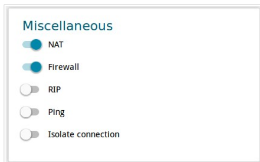
Figure 67. The page for creating a new PPPoE connection. The Miscellaneous section.
