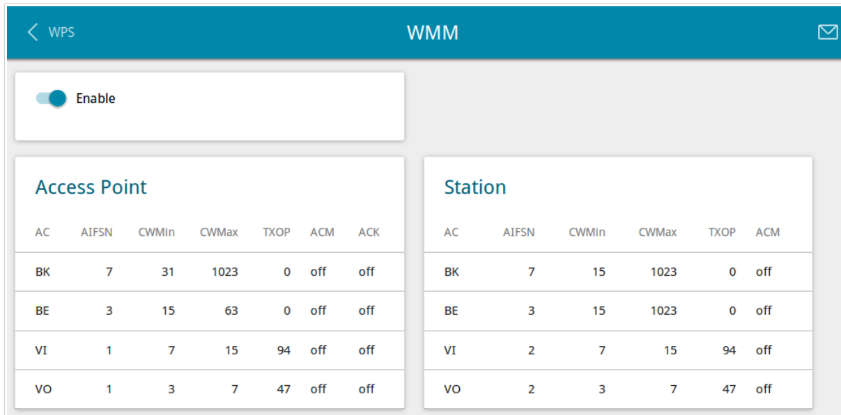
Figure 89. The page for configuring the WMM function.
