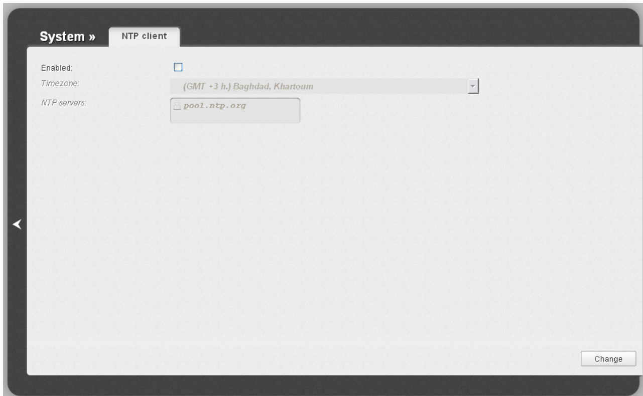
Figure 130. The System / NTP client page.
