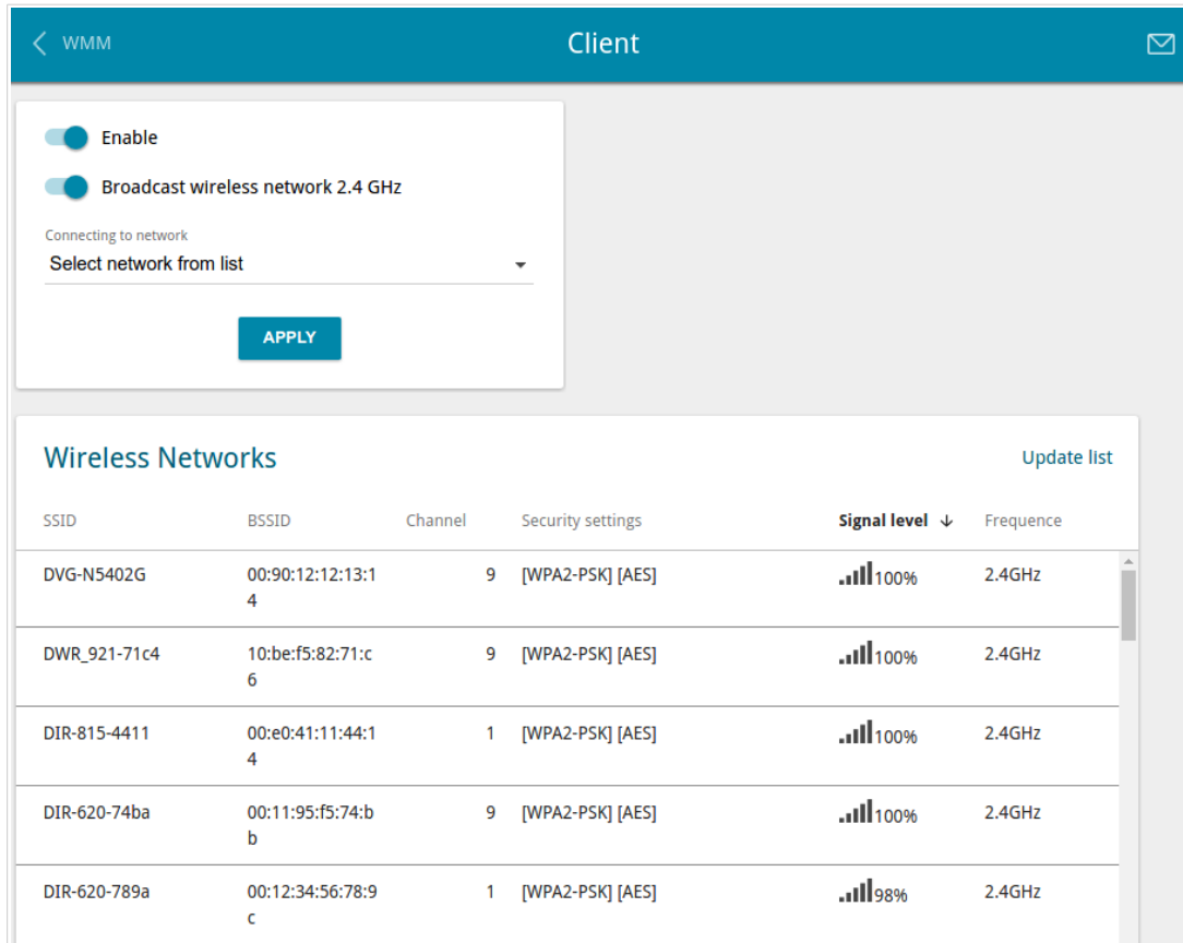
Figure 88. The page for configuring the client mode.
