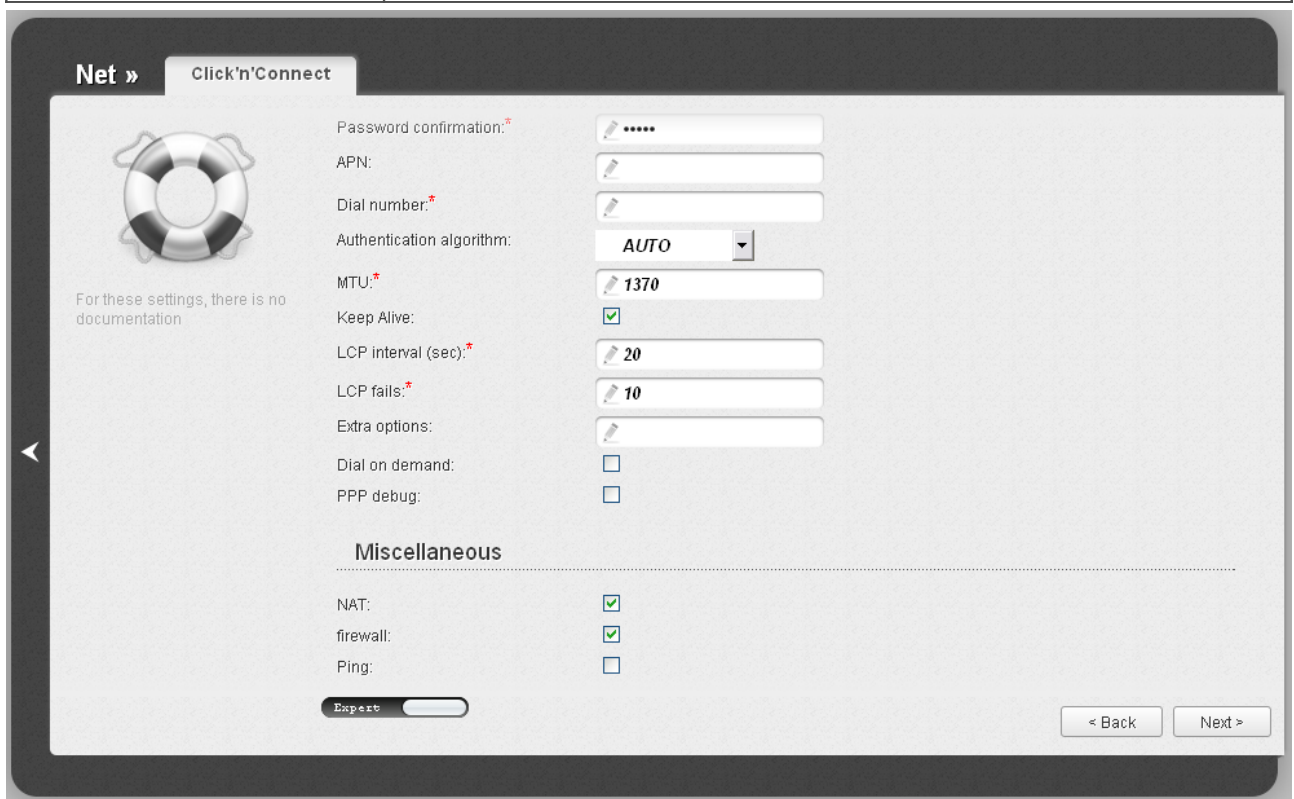
Figure 55. Configuring 3G WAN connection. The expert settings mode. The Miscellaneous section.
