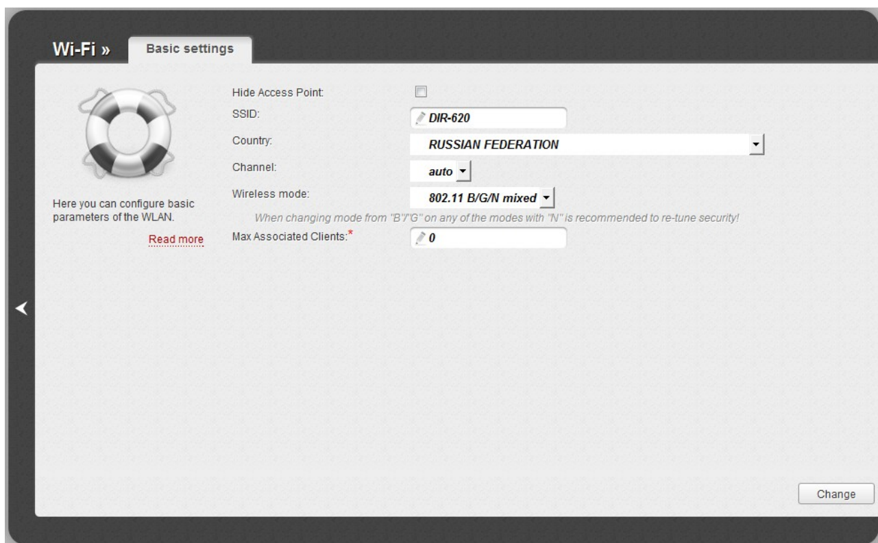
Figure 98. Basic settings of the wireless LAN.
