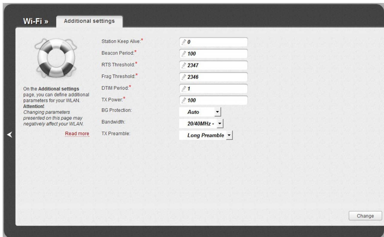
Figure 108. Additional settings of the WLAN.
