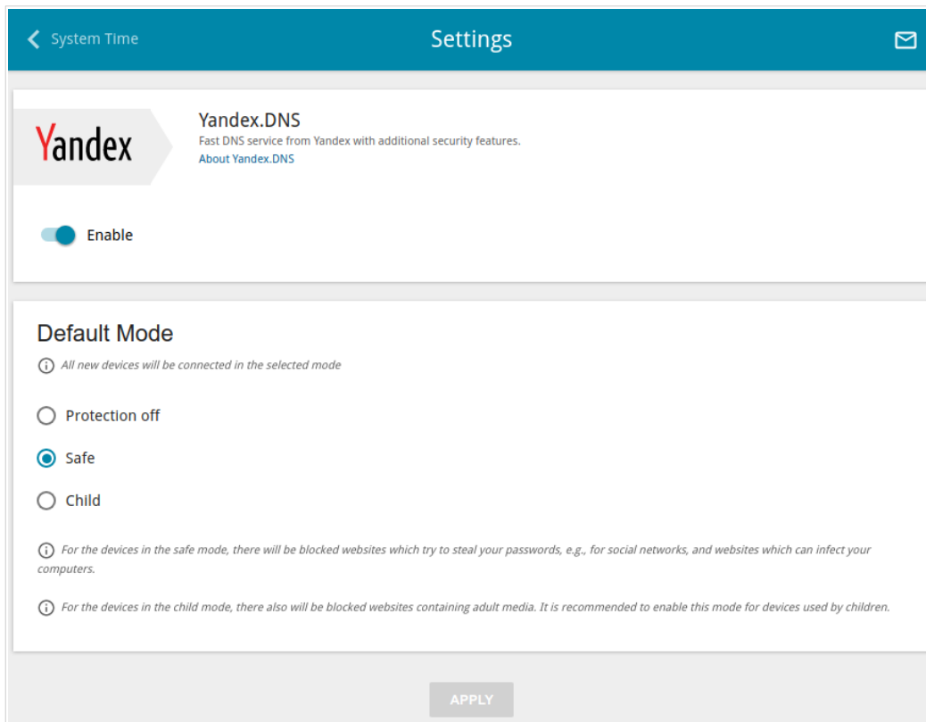
Figure 144. The Yandex.DNS / Settings page.
