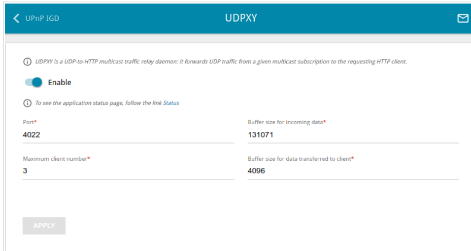
Figure 117. The Advanced / UDPXY page.
