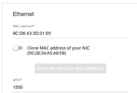
Figure 54. The page for creating a new Static IPv4 connection. The Ethernet section.
