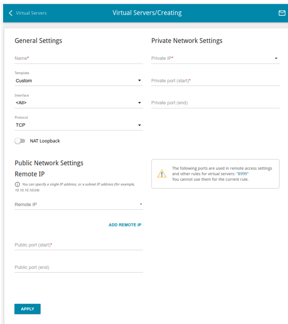
Figure 128. The page for adding a virtual server.
