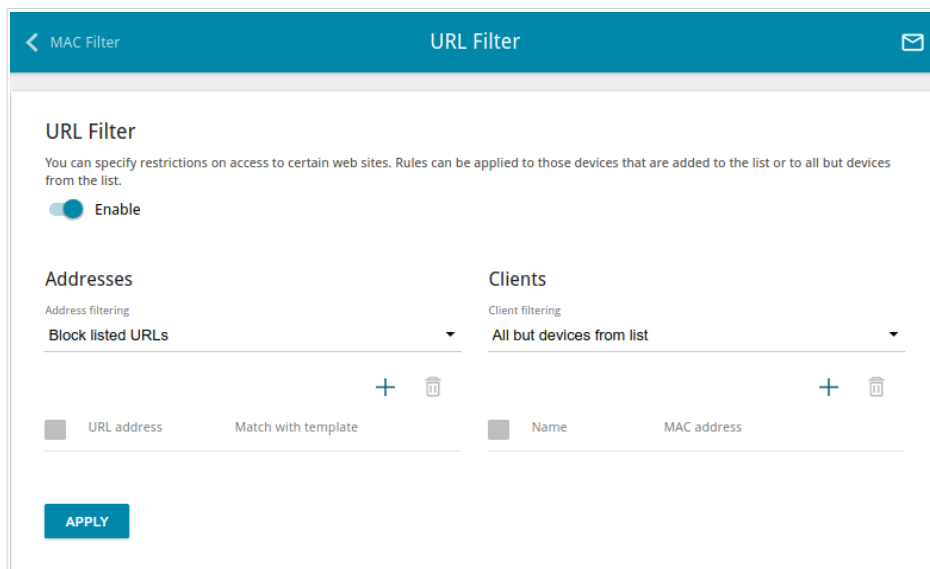
Figure 132. The Firewall / URL Filter page.
