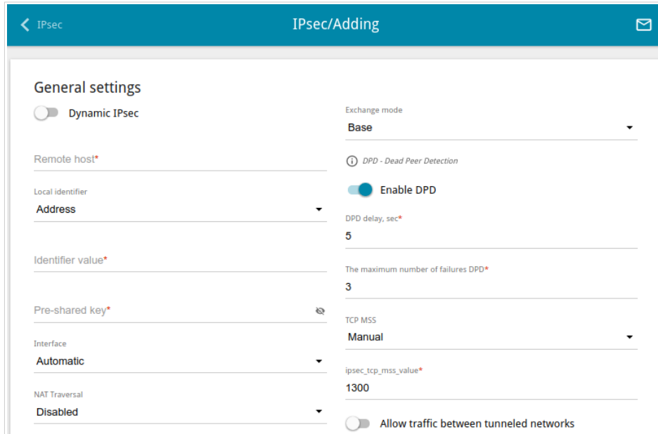
Figure 122. The page for adding an IPsec tunnel. The General settings section.
