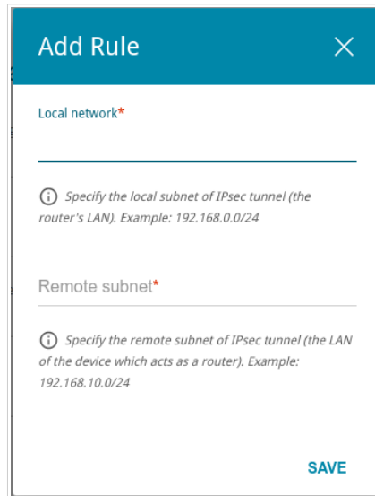
Figure 124. The page for adding an IPsec tunnel. The window for adding a tunneled network.
