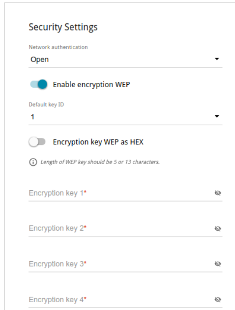
Figure 86. The Open value is selected from the Network authentication drop-down list.
