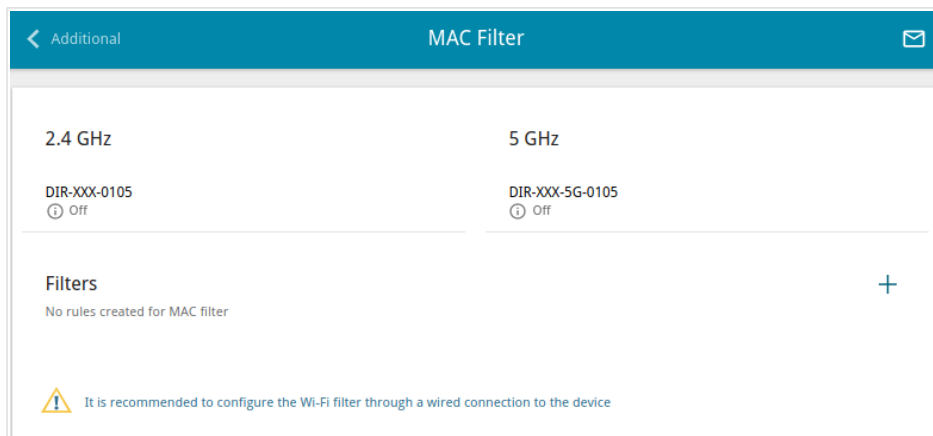
Figure 97. The page for configuring the MAC filter for the wireless network.
