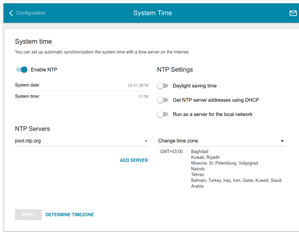
Figure 143. The System / System Time page.
