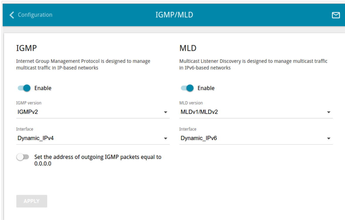
Figure 119. The Advanced / IGMP/MLD page.
