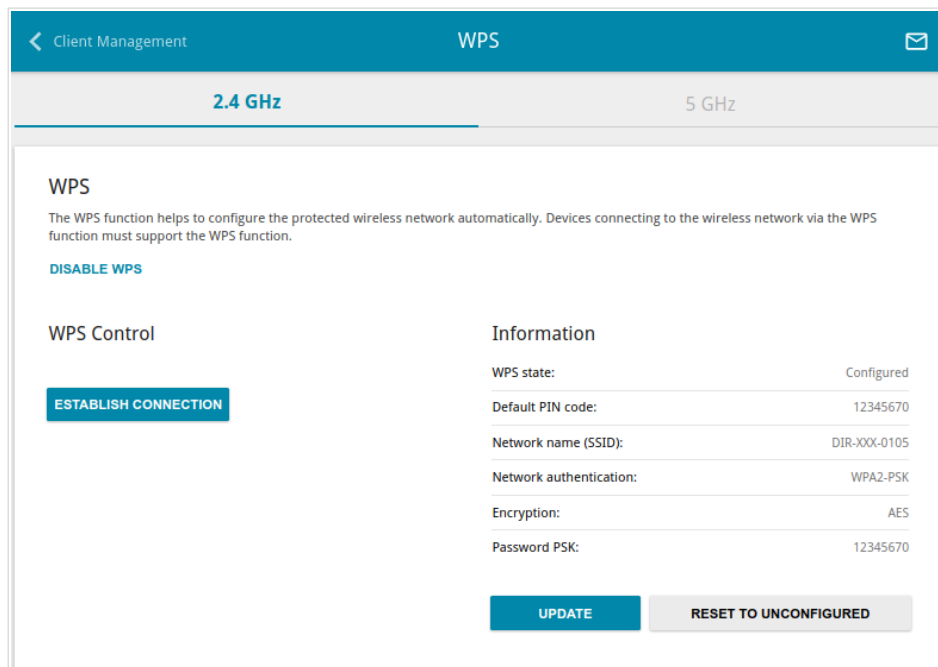
Figure 90. The page for configuring the WPS function.
