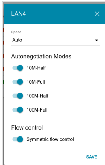
Figure 107. The window for changing the settings of the router's port.
