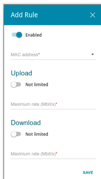
Figure 95. The window for setting up rate limit.
