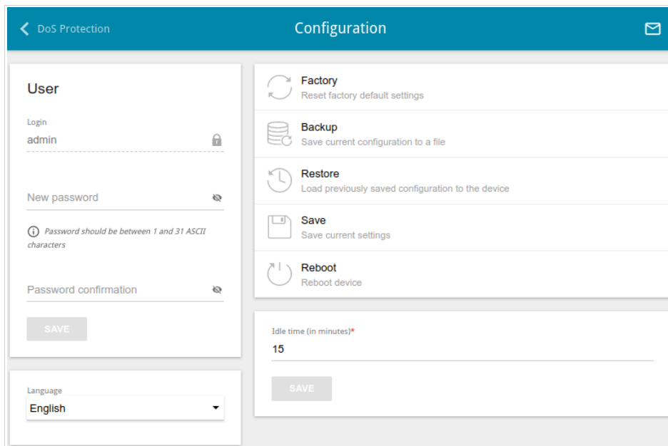
Figure 134. The System / Configuration page.
