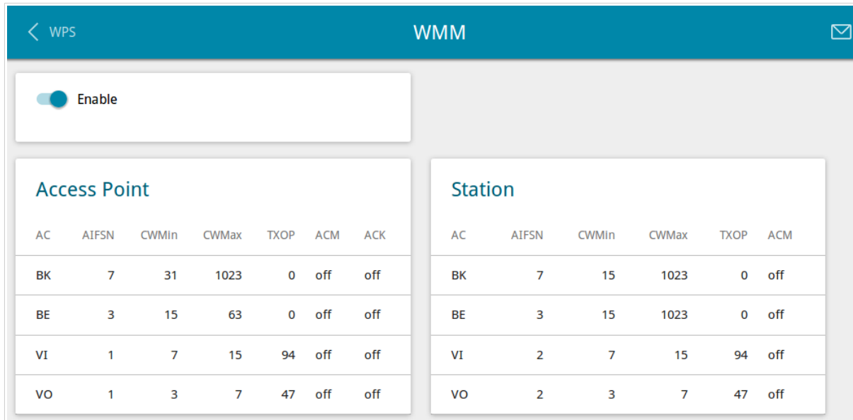
Figure 101. The page for configuring the WMM function.
