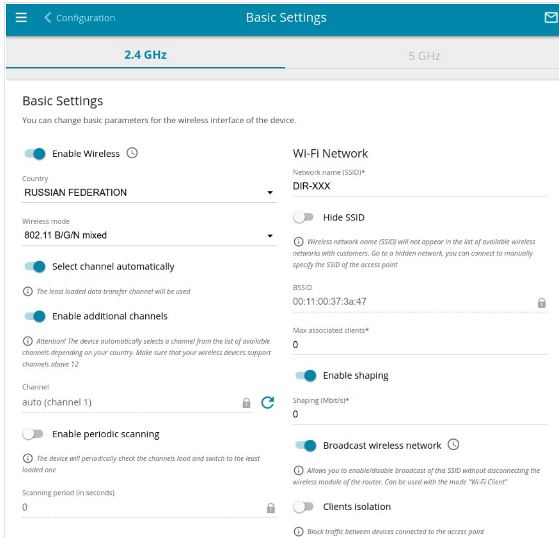
Figure 109. Basic settings of the wireless LAN in the 2.4GHz band.
