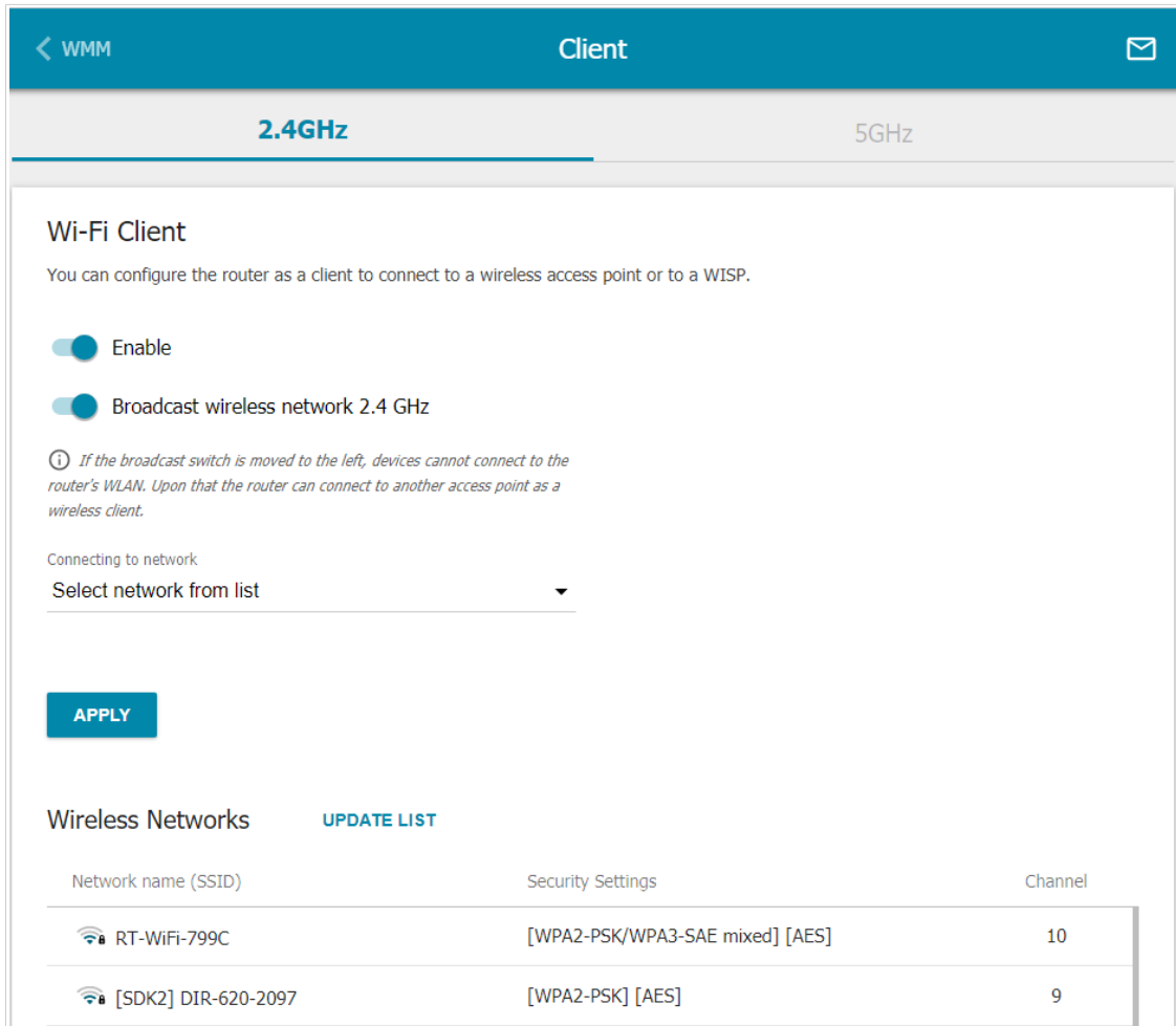
Figure 119. The page for configuring the client mode.
