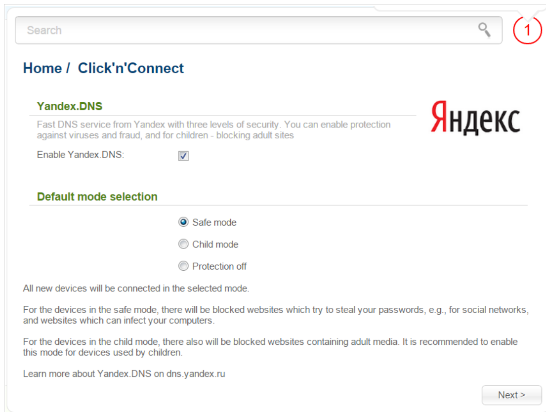
Figure 45. Configuring the Yandex.DNS service.
