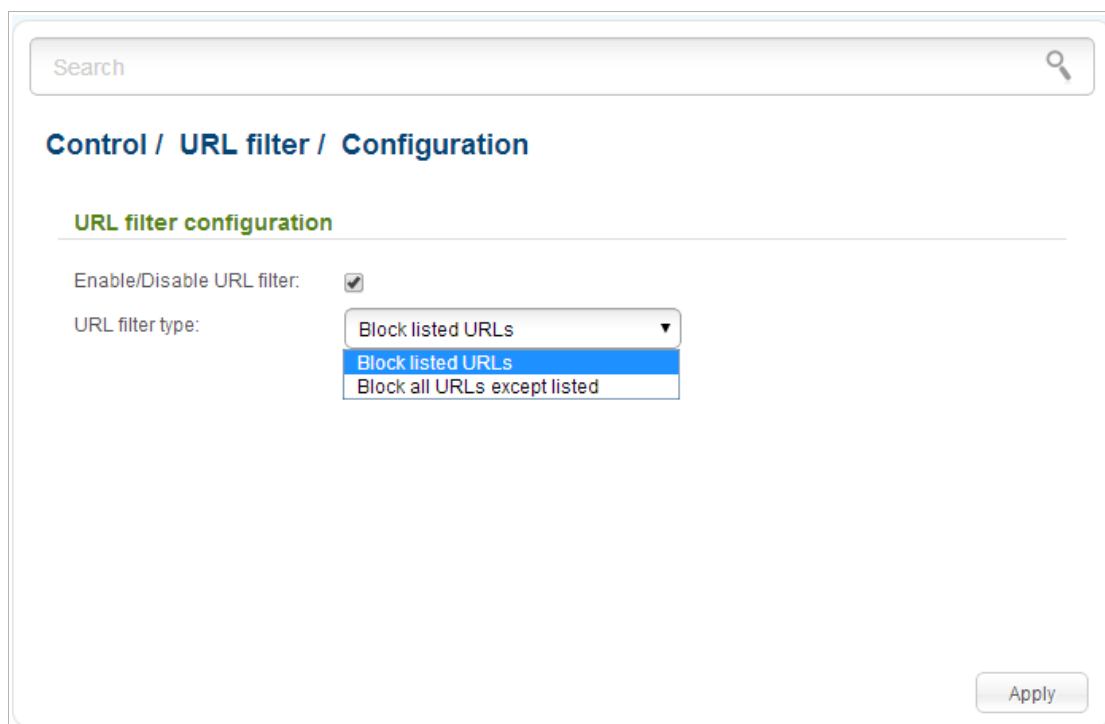
Figure 155. The Control / URL filter / Configuration page.
