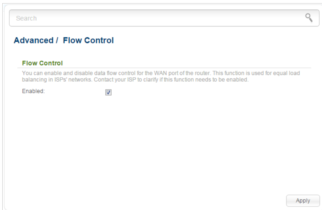
Figure 133. The Advanced / Flow Control page.
