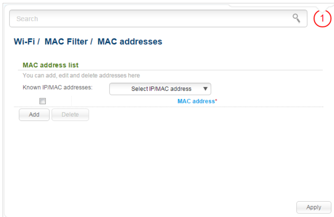
Figure 117. The page for adding a MAC address.
