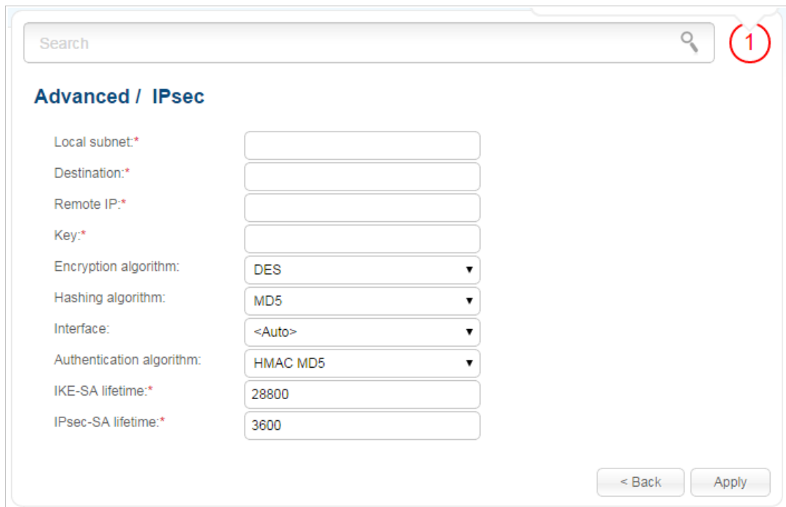
Figure 135. The page for adding a VPN tunnel.
