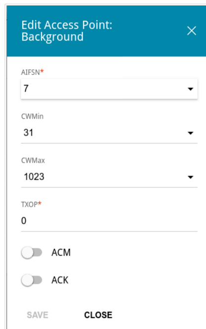
Figure 108. The window for changing parameters of the WMM function.
