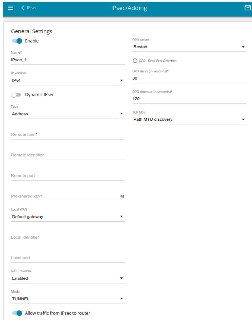
Figure 135. The page for adding an IPsec tunnel. The General Settings section.
