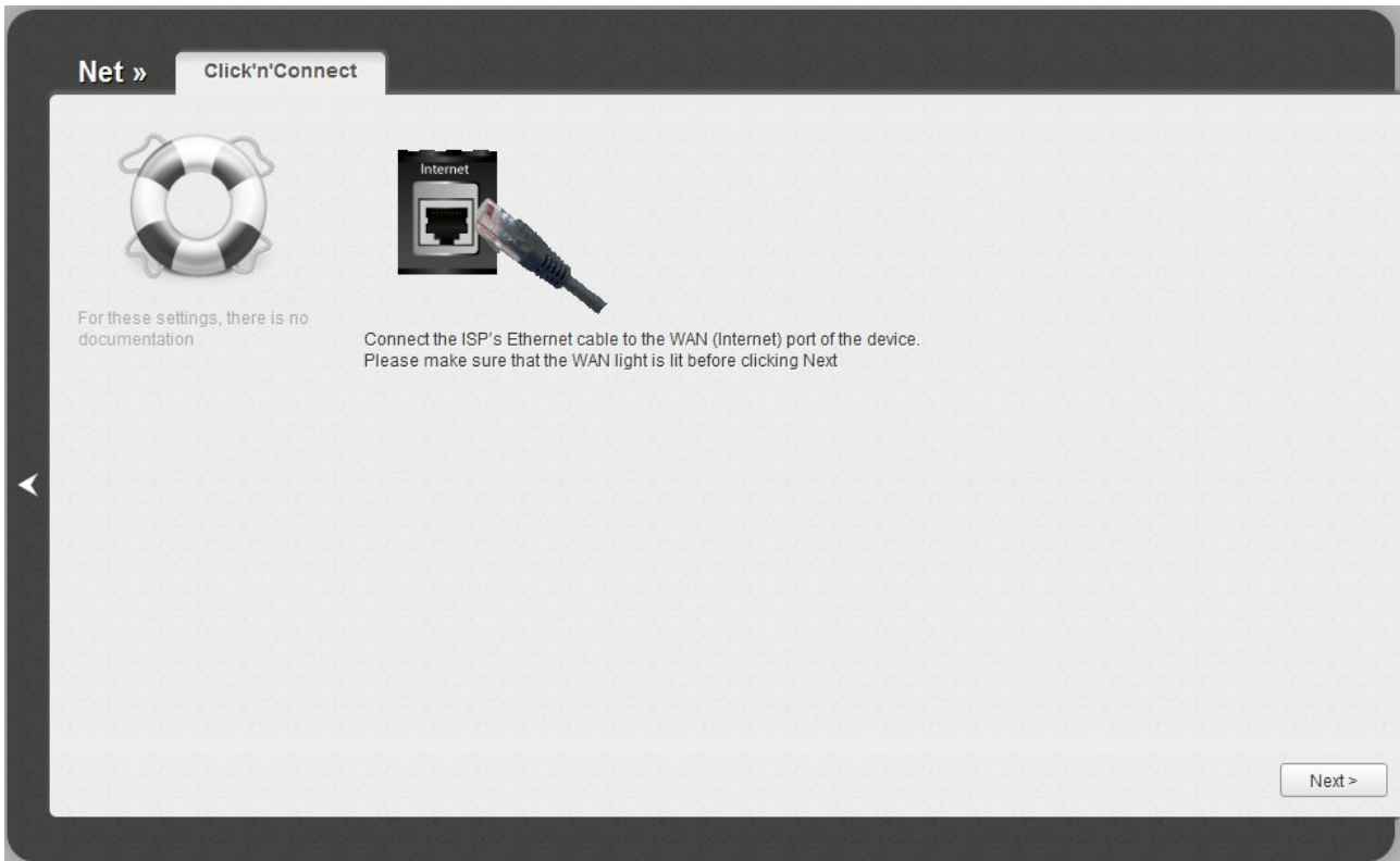
Figure 27. Configuring a WAN connection.
