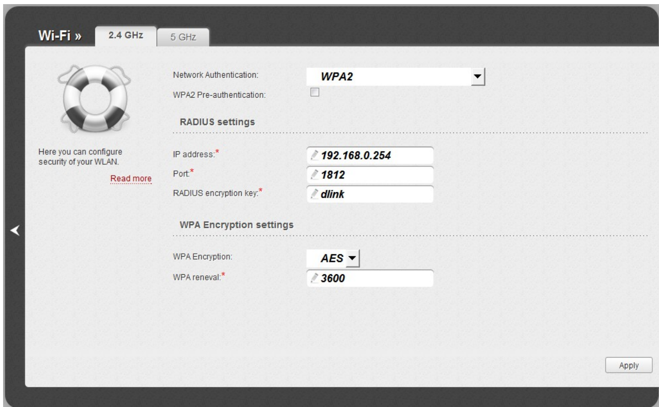
Figure 94. The WPA2 value is selected from the Network Authentication drop-down list.
