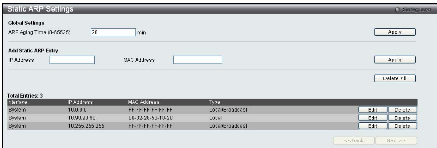
Figure 2 - 11. Static ARP Settings window
