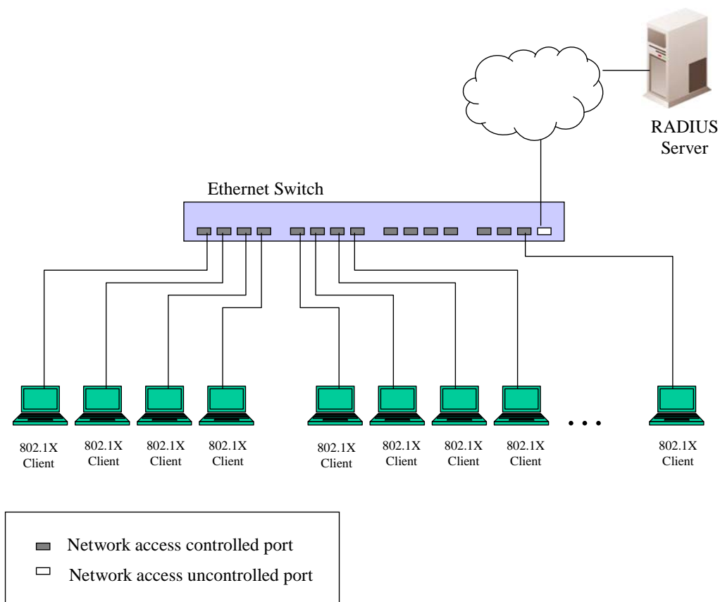
Figure 5 - 17. Example of Typical Port-based Configuration
