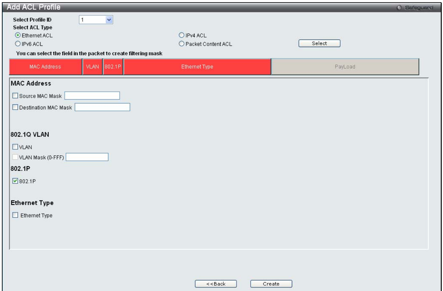
Figure 6 - 47. Add ACL Profile window for Ethernet example
