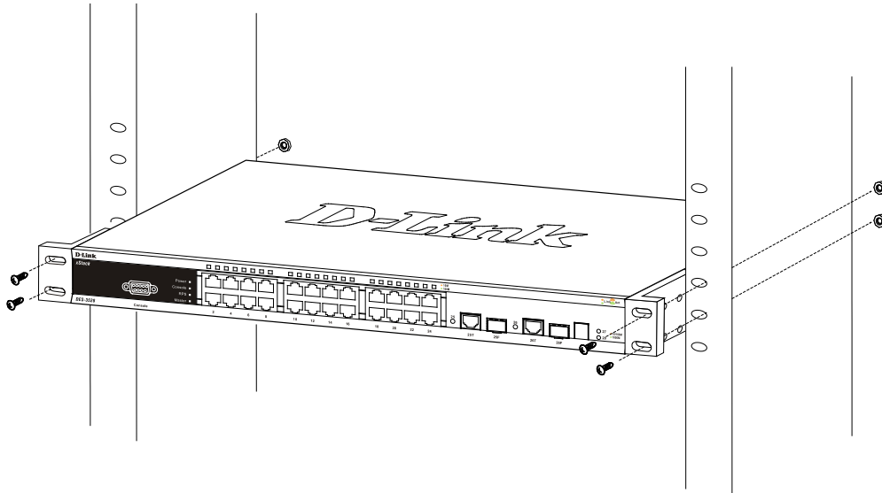
Figure 2- 4. Installing the Switch in a rack (front)
