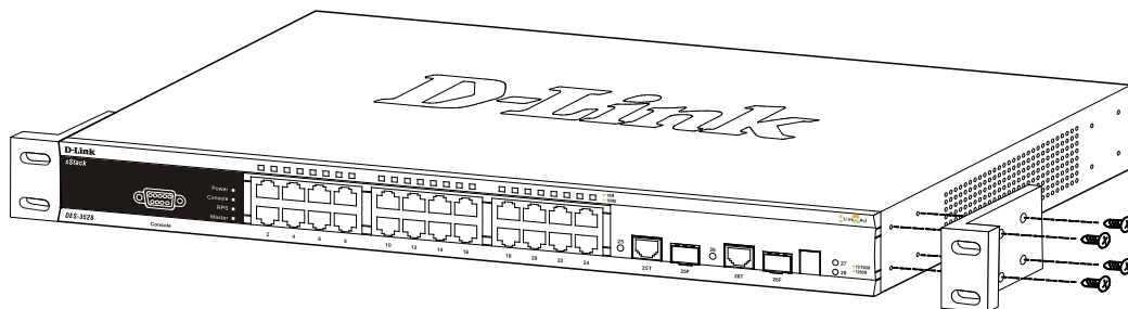
Figure 2- 2. Fasten mounting brackets to the Switch (front)
