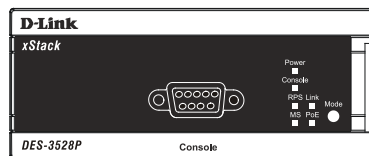
Figure 1- 9. LED Indicators on DES-3528P switch
