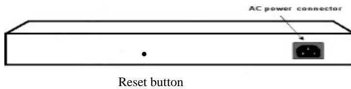
Figure 5 – Rear panel of the Switch
