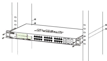
Figure 4. Installing the switch in a standard-sized equipment rack
