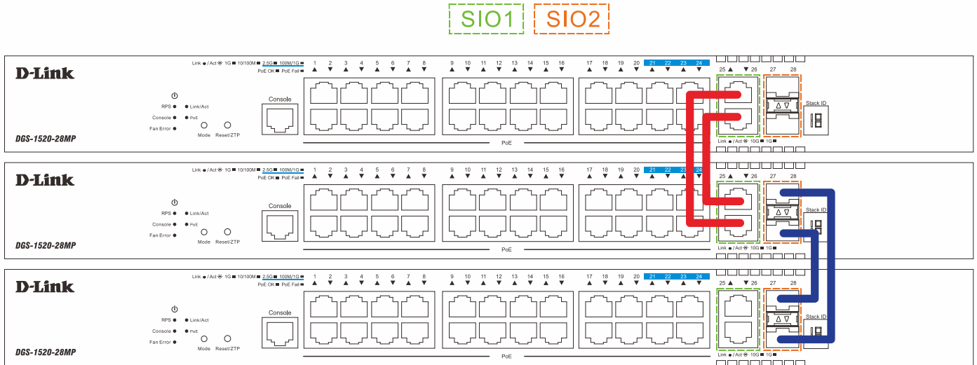
Figure 4-88 Duplex Chain Stacking Topology (Odd, 4-port)
