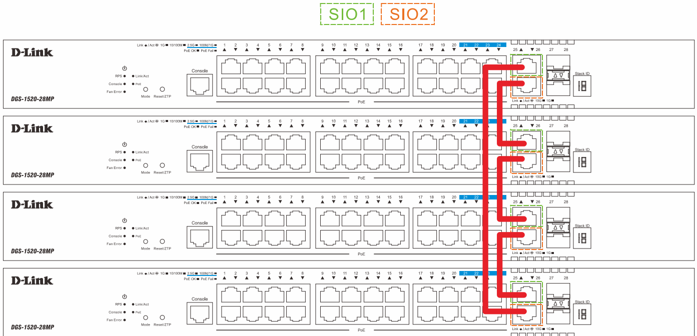
Figure 4-85 Duplex Ring Stacking Topology (Even, 2-port)
