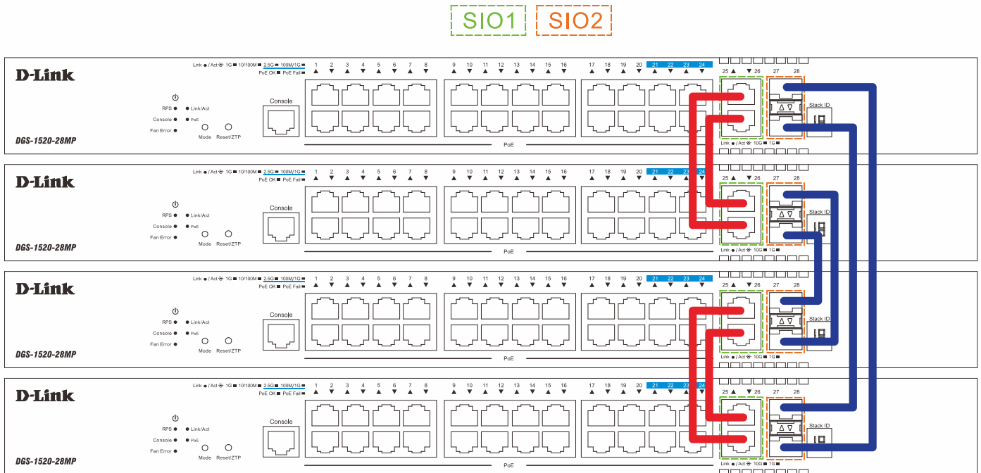
Figure 4-87 Duplex Ring Stacking Topology (Even, 4-port)
