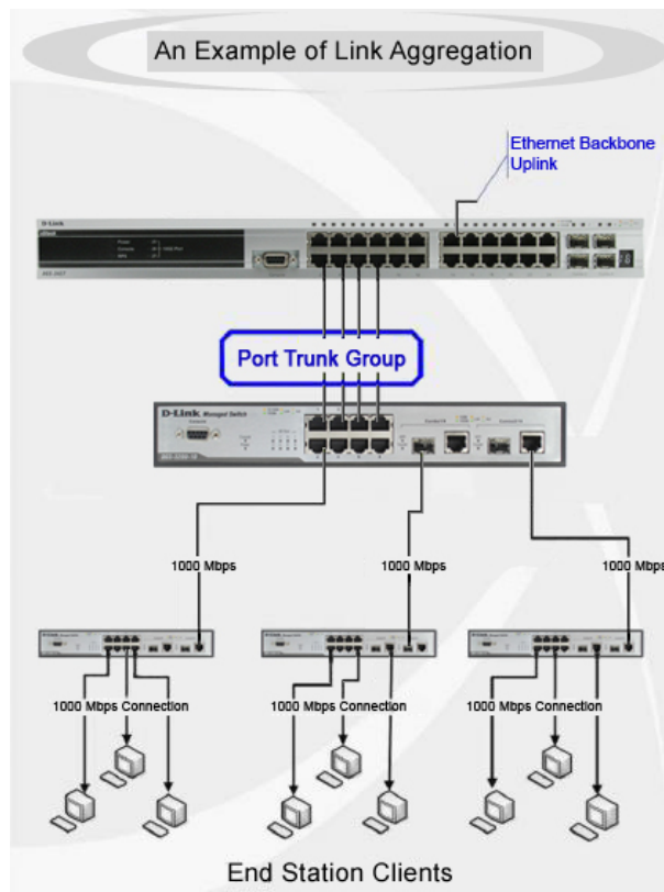
Figure 5-67 Example of Port Trunk Group
