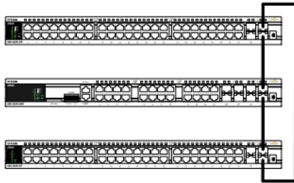
Figure 2-32 Switches stacked in a Duplex Ring
