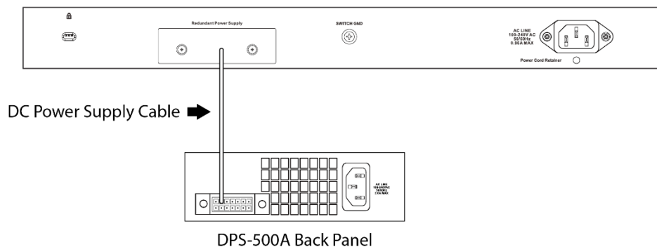
Figure 3-9 Connecting a DXS-3130-28 and DXS-3130-32S Switch to the DPS-500A
