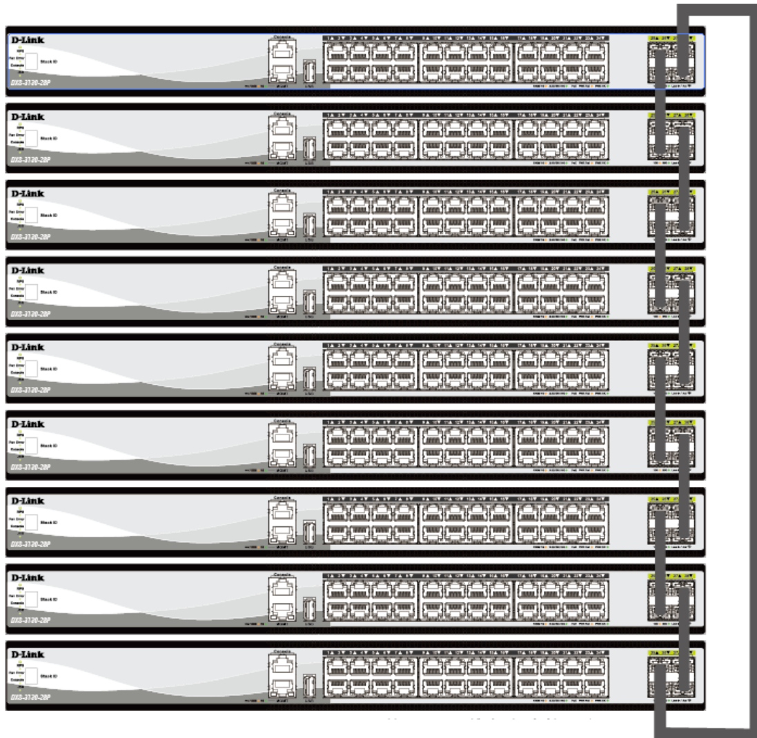
Figure 0-4 Duplex Ring stacking topology (SFP28 ports)
