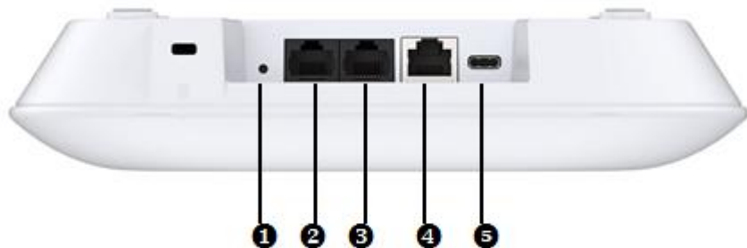
Figure 2: Rear Connectors
